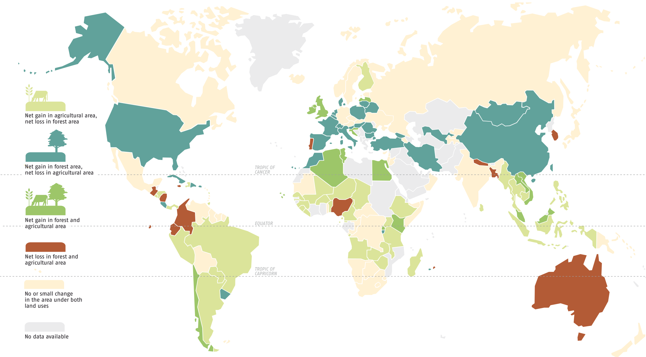
TRENDS IN LAND-USE CHANGE Net changes in agricultural and forest areas, by country/territory, 2000–2010
